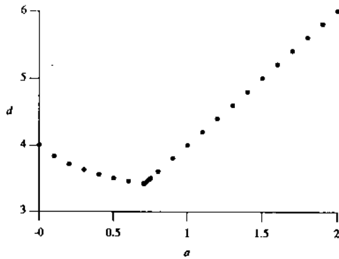
Fig. 2. Max-min distance found by the numerical search algorithms for the channel h(D) = 1 + aD + D^2 .
